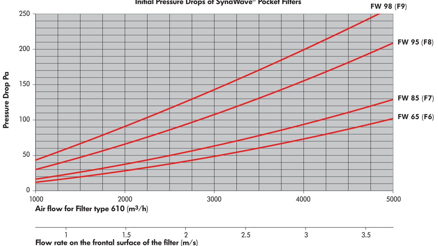
Initial Pressure Drops of SynaWave® Pocket Filters
